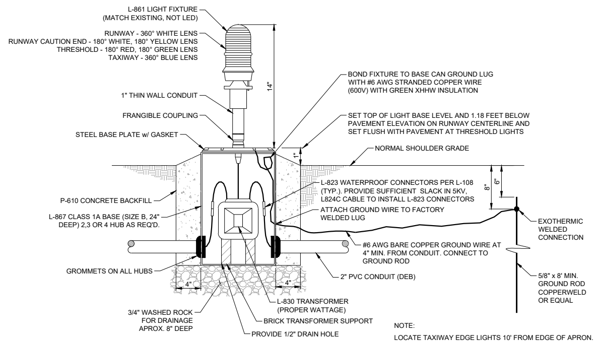
5 BASE MOUNTED L-861 LIGHT 5.2 NOT TO SCALE (MIRL CIRCUIT)
