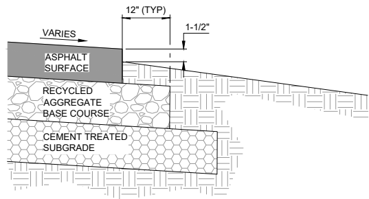
3 ASPHALT EDGE 4.1 NOT TO SCALE
