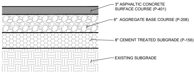
2 APRON TYPICAL SECTION 4.1 NOT TO SCALE
