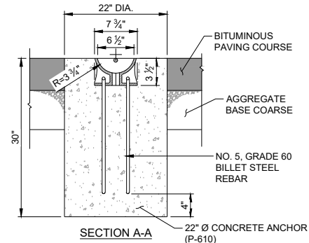
3 AIRCRAFT TIEDOWN DETAIL 6.1 NOT TO SCALE
