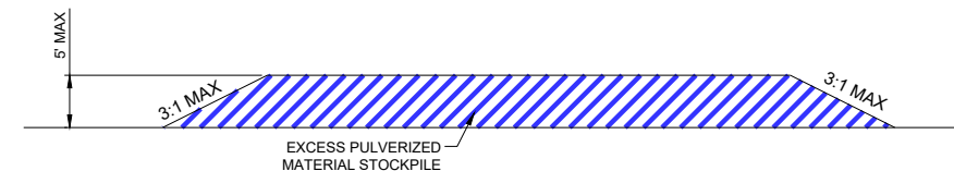
5 STOCKPILE NOT TO SCALE
