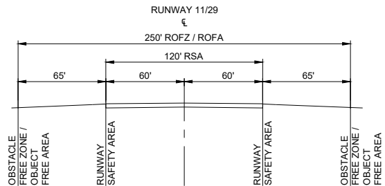
2 SAFETY AREAS NOT TO SCALE
