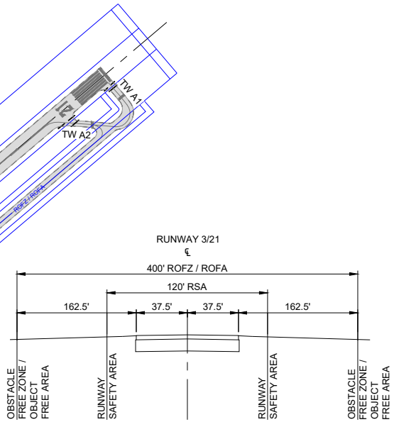
2 SAFETY AREAS NOT TO SCALE
