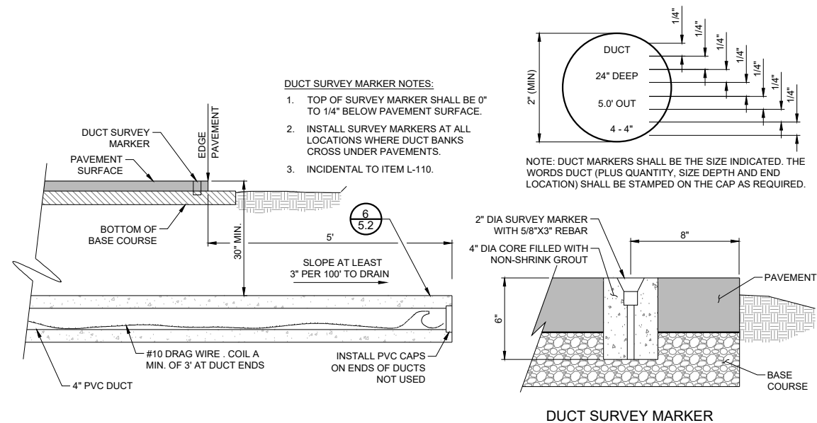
4 DUCT & DUCT MARKER 5.2 NOT TO SCALE
