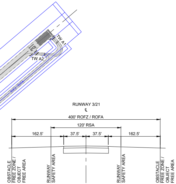
2 SAFETY AREAS NOT TO SCALE
