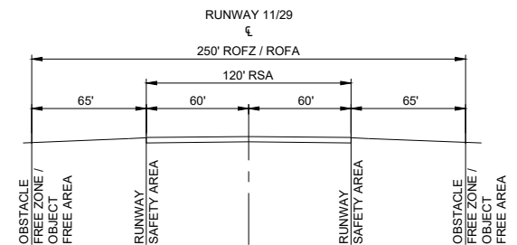
2 SAFETY AREAS NOT TO SCALE
