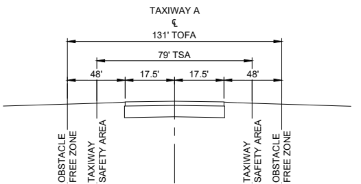
3 SAFETY AREAS NOT TO SCALE
