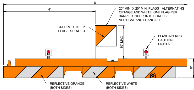
1 LOW PROFILE SAFETY BARRIER NOT TO SCALE
