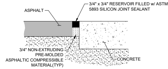
4 CONCRETE / ASPHALT JOINT SEAL 4.1 NOT TO SCALE
