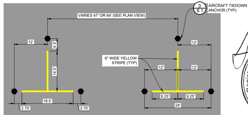
2 TIEDOWN MARKING DETAIL 6.1 NOT TO SCALE
