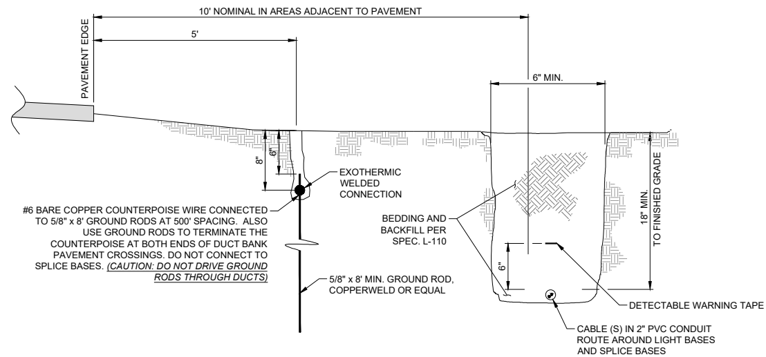
1 TRENCH & CABLE PLACEMENT 5.2 NOT TO SCALE
