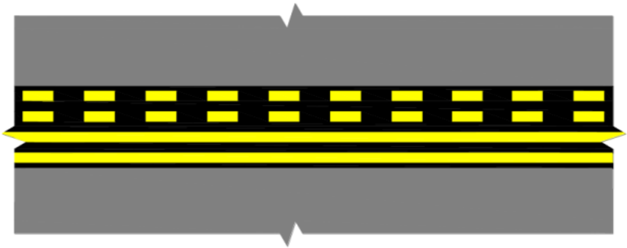
Runway Holding Position Marking
