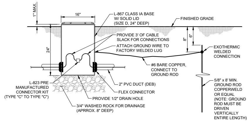
3 SPLICE BASE DETAIL (L-867) 5.2 NOT TO SCALE
