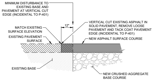
1 JOINT AT EXISTING PAVEMENT EDGE 4.1 NOT TO SCALE
