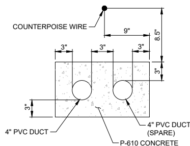
6 2-WAY DUCT BANK 5.2 NOT TO SCALE
