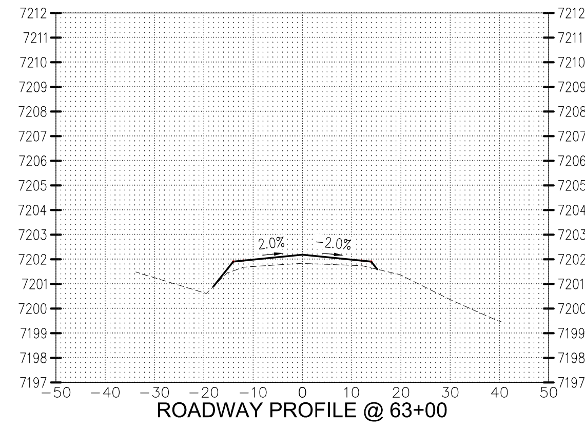
ROADWAY PROFILE @ 63+00
