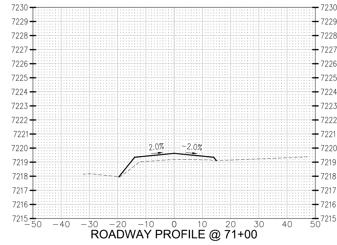
ROADWAY PROFILE @ 71+00
