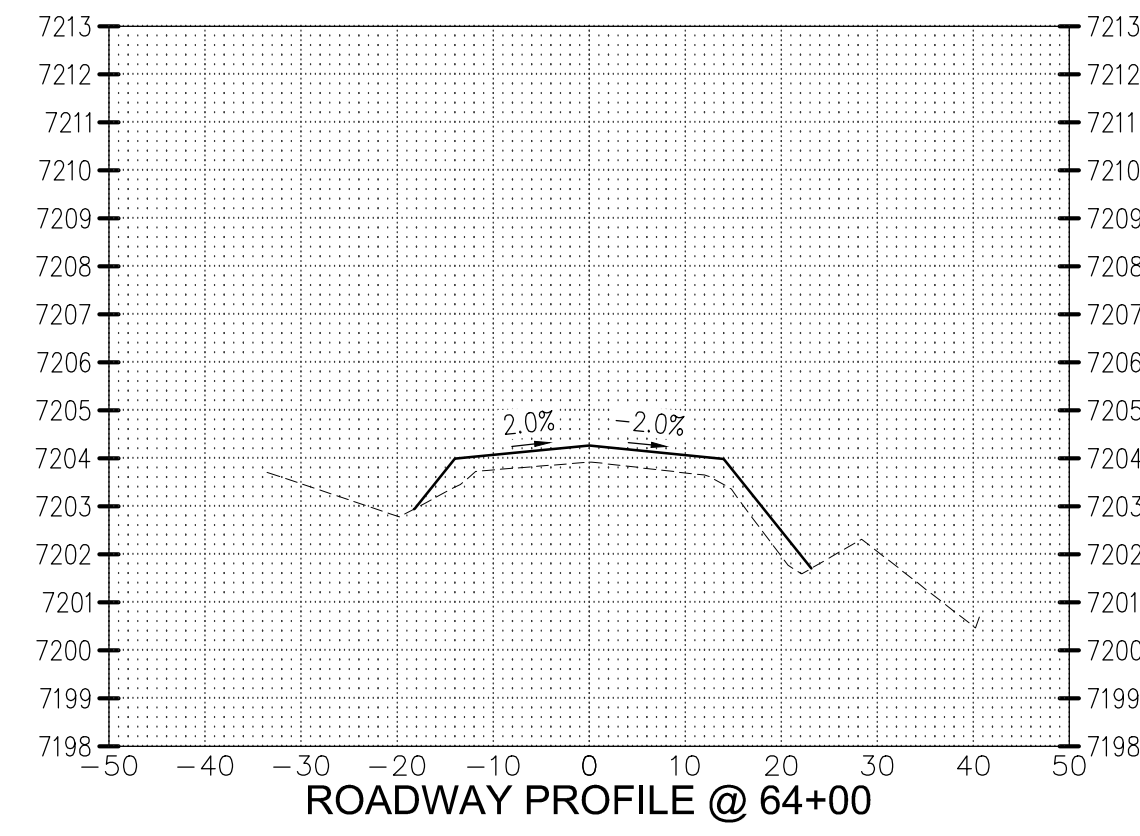
ROADWAY PROFILE @ 64+00
