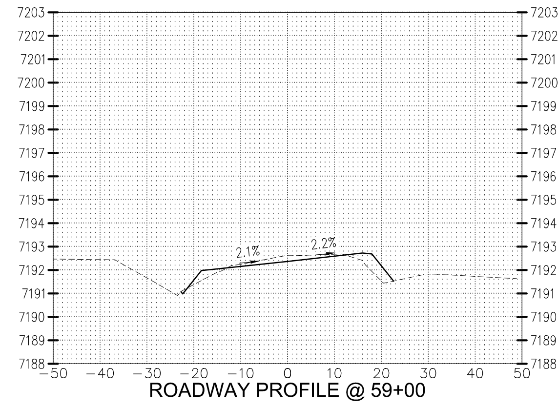
ROADWAY PROFILE @ 59+00
