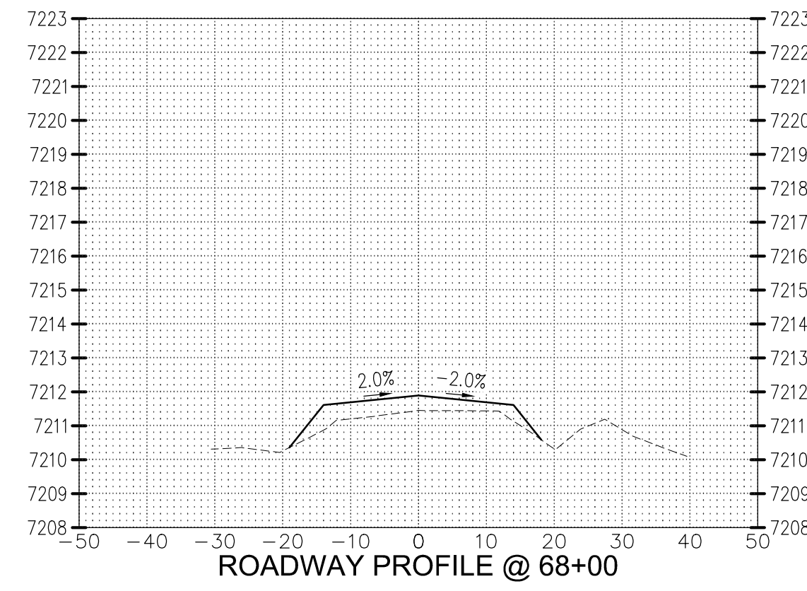
ROADWAY PROFILE @ 68+00
