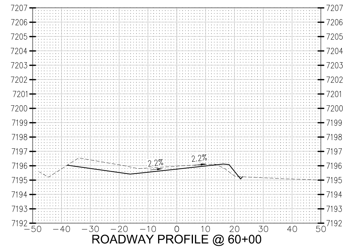
ROADWAY PROFILE @ 60+00
