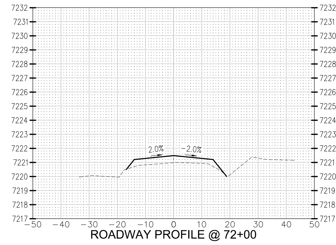
ROADWAY PROFILE @ 72+00
