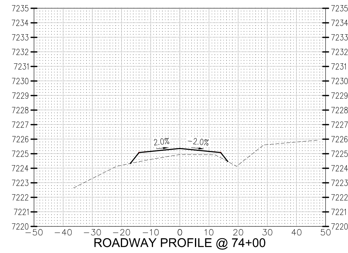
ROADWAY PROFILE @ 74+00
