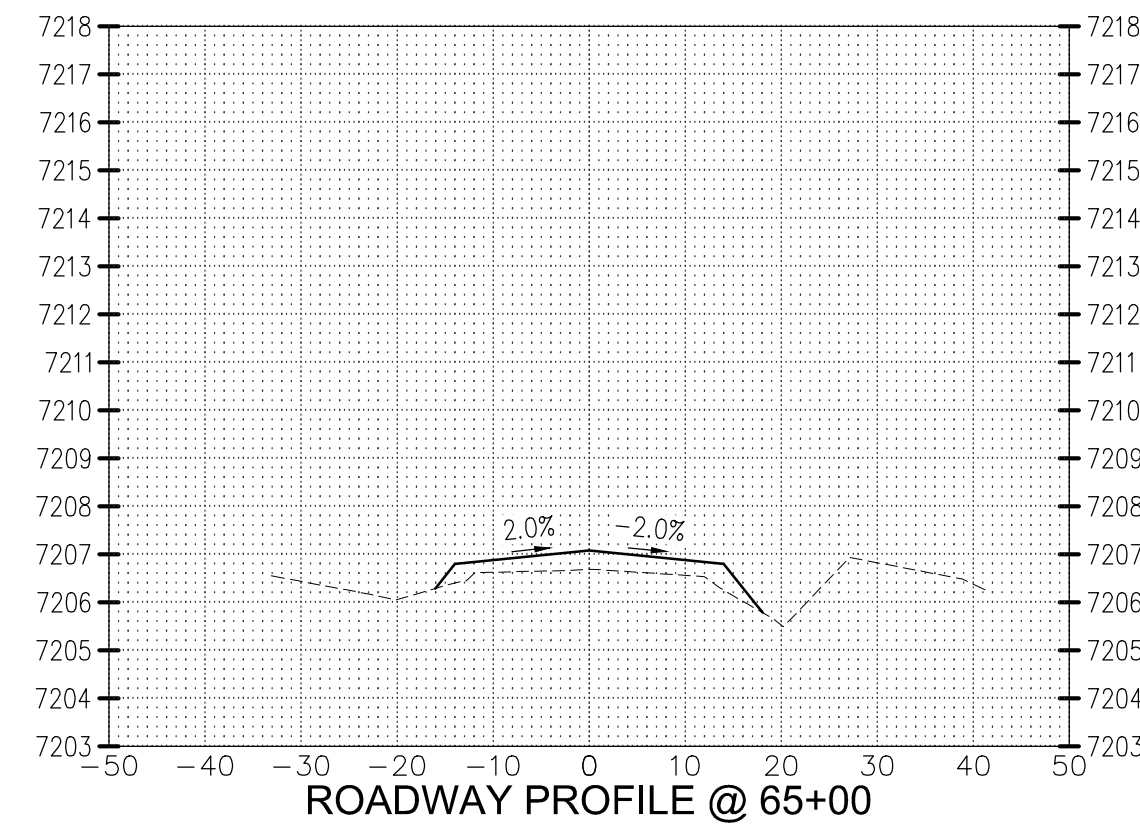
ROADWAY PROFILE @ 65+00
