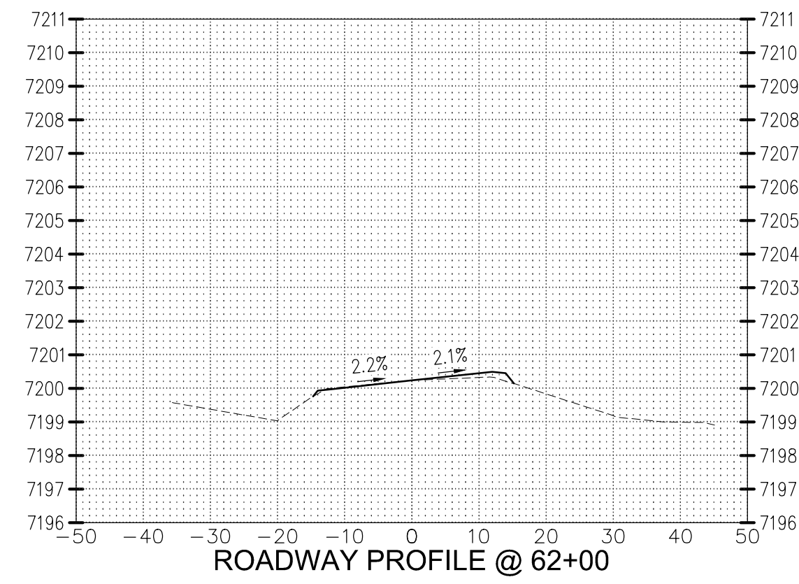
ROADWAY PROFILE @ 62+00
