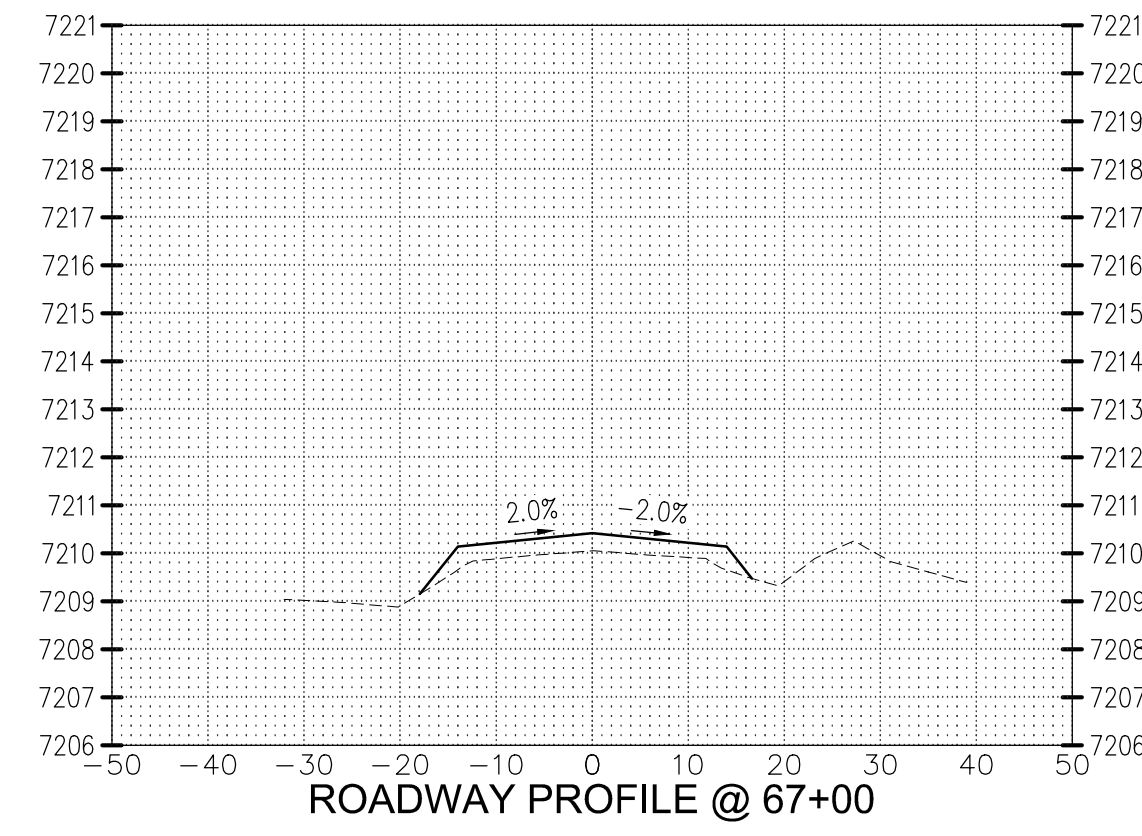
ROADWAY PROFILE @ 67+00
