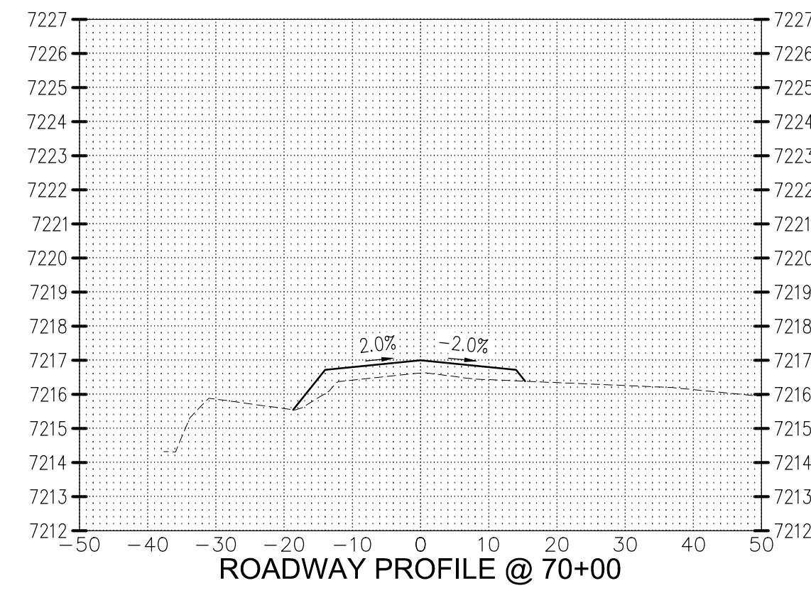
ROADWAY PROFILE @ 70+00
