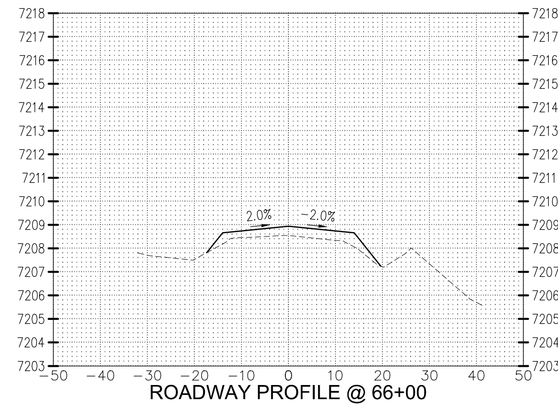
ROADWAY PROFILE @ 66+00
