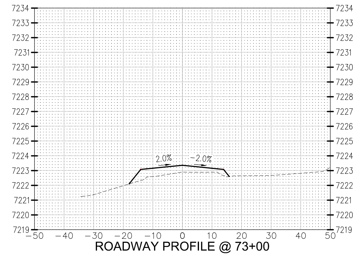
ROADWAY PROFILE @ 73+00
