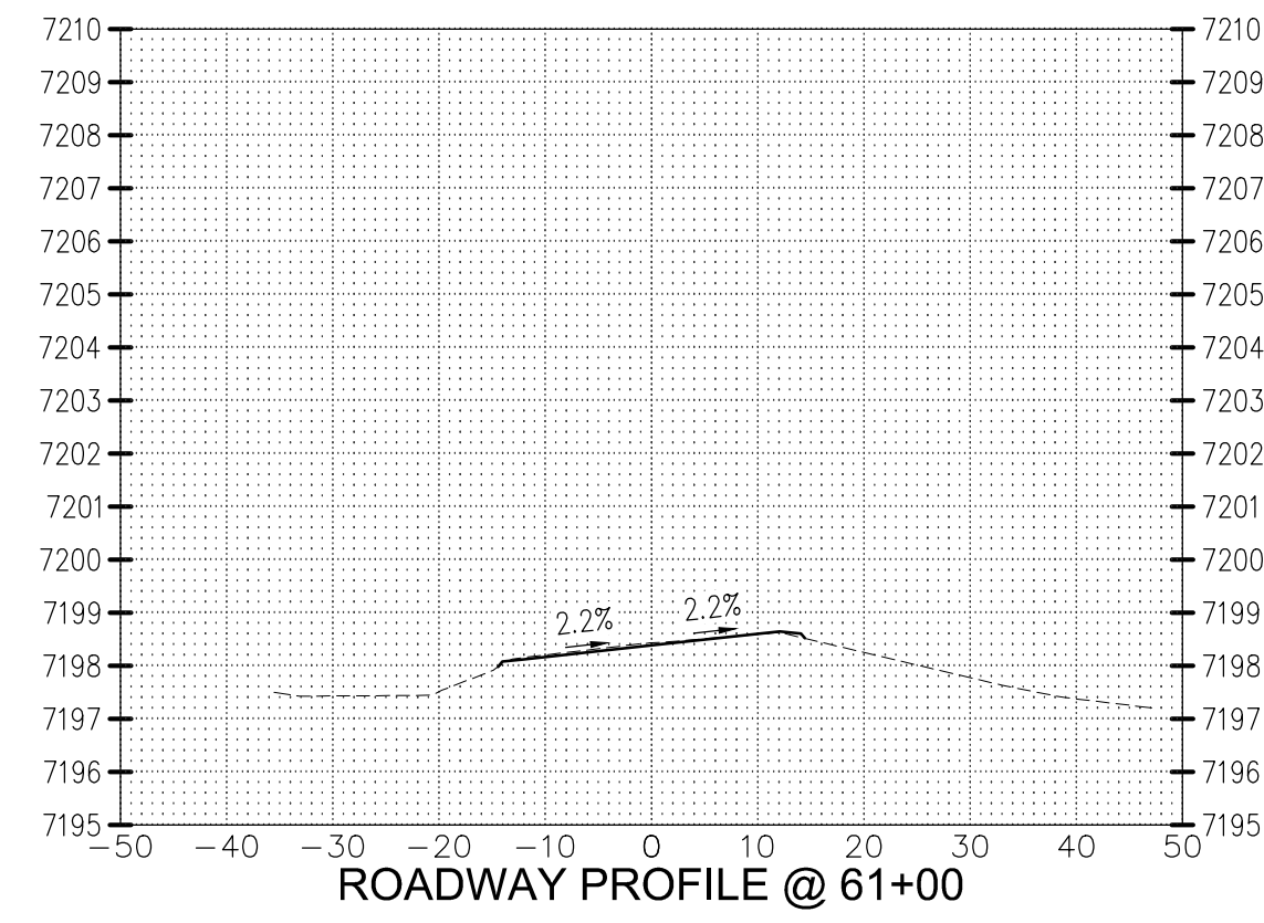
ROADWAY PROFILE @ 61+00
