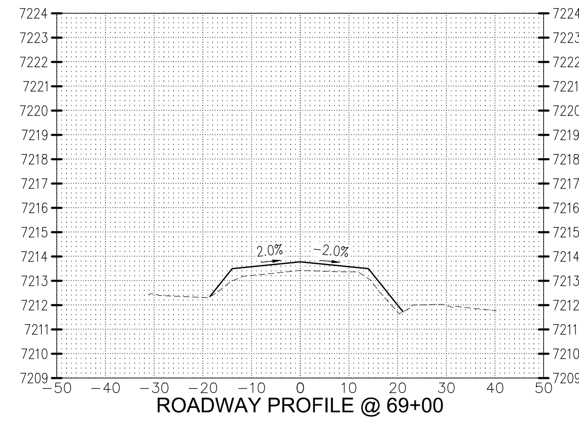
ROADWAY PROFILE @ 69+00
